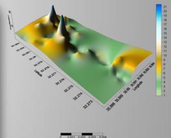
Amplification Factor surface map for JERASH City
