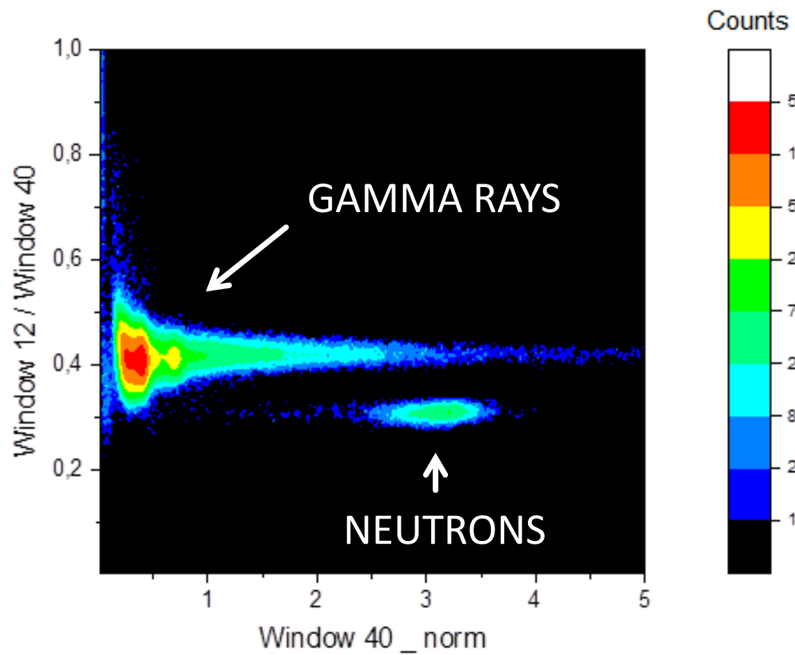
Fig.6: PSD CLYC PSD intensity plots with a 252 Cf source. Windows were set [0,12] and [12,40] with a channel width of 10 ns.
