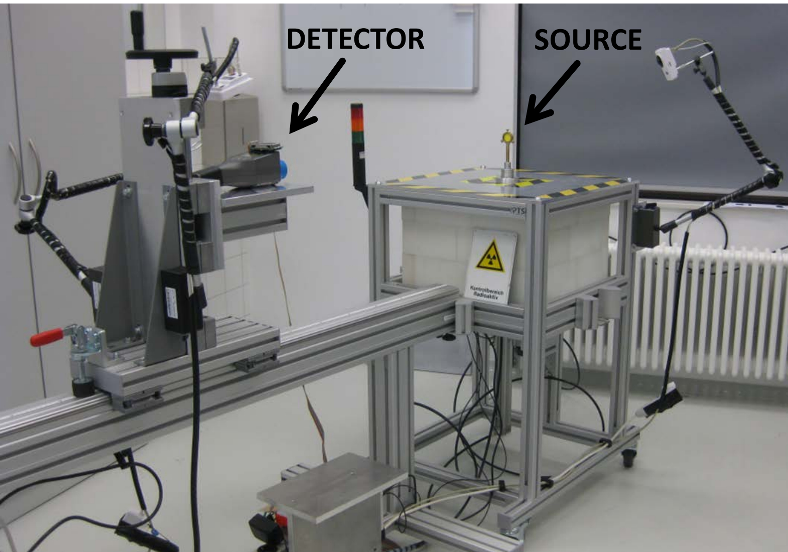
Fig.2: Static test system Picture of the static test system.
