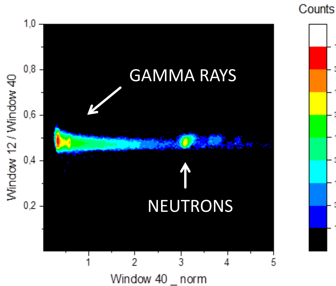
Fig.8: PSD CLLB PSD intensity plots with a 252 Cf source. Windows were set [0,12] and [12,40] with a channel width of 10 ns.
