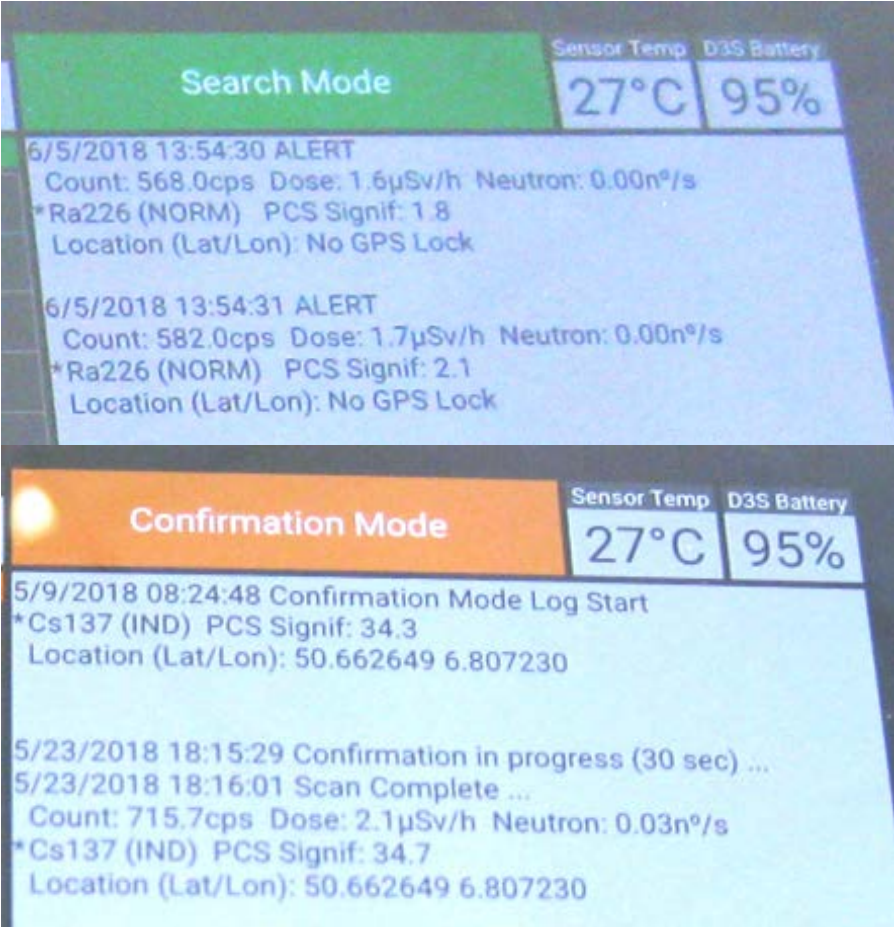
Fig.4: Operational Modes D3S The upper picture shows a screenshot of D3S in Search Mode. The lower picture shows a screenshot of D3S in Confirmation Mode.
