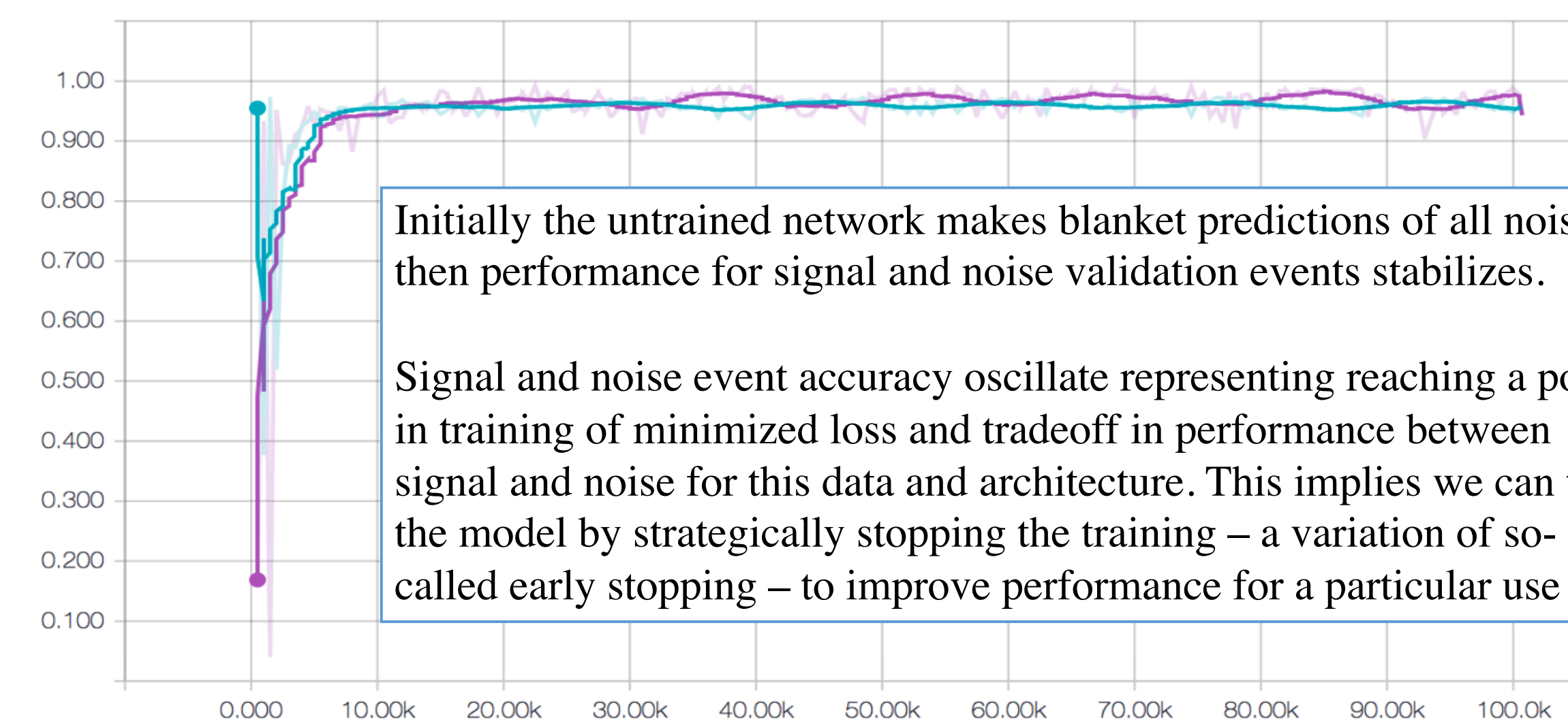
Figure 3: Detection accuracy of noise (purple) and signal events (blue).
